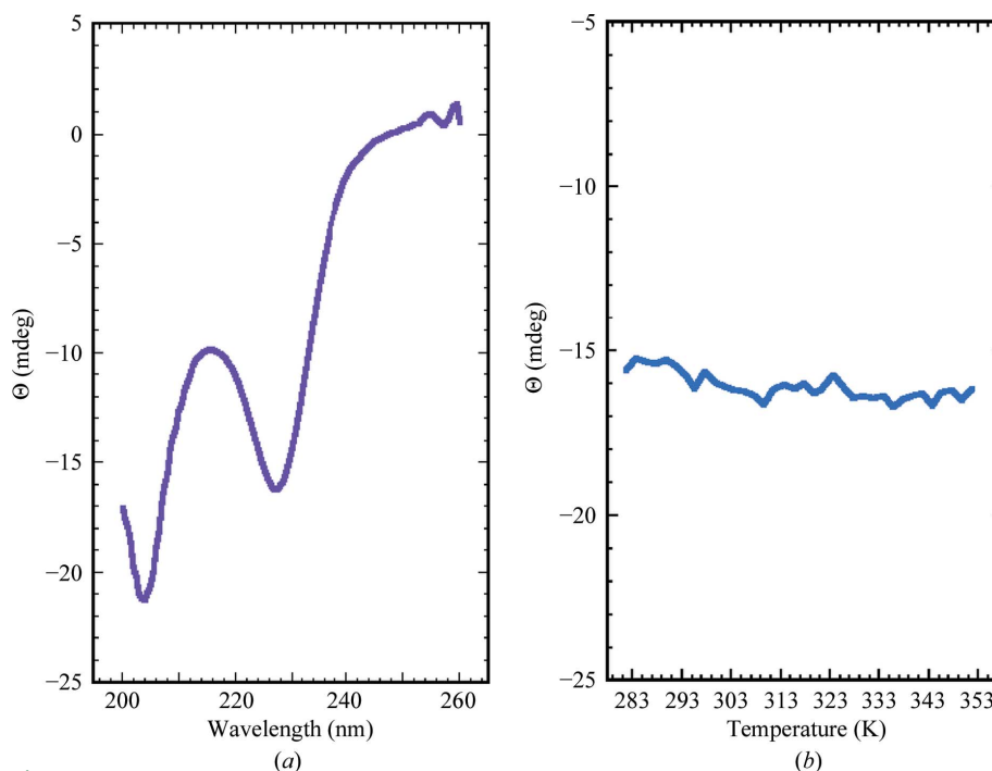
Figure 4 (a) Circular dichroism steady-state wavelength spectrum of Mt -RubB ( \sim 0.05 mM) in NMR buffer collected at 298 K. (b) The CD thermal plot for Mt -RubB obtained by measuring the ellipticity at 226 nm in 2.0 K intervals between 283 and 353 K.
